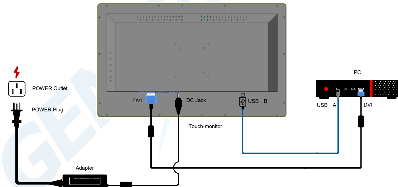
Fig 10 Touch Monitor Connection Diagram 1
