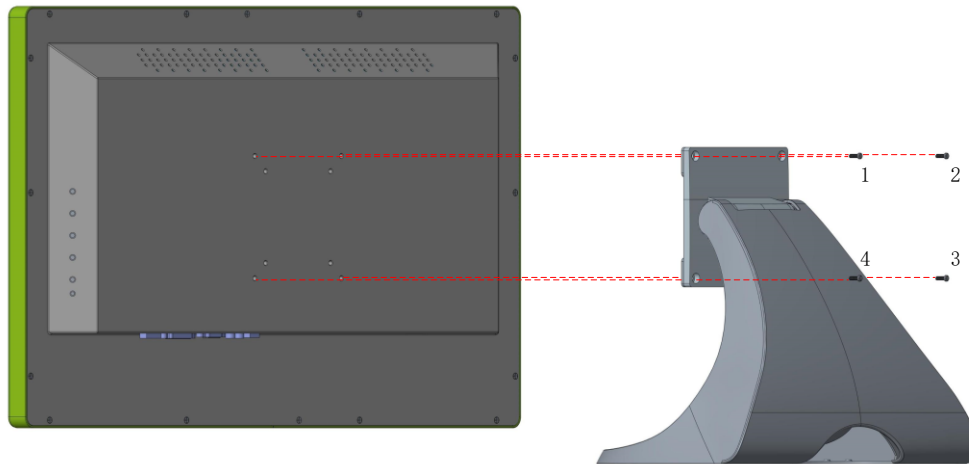
Fig 4 Desktop Installation Diagram (Using 23.8" as an Example)
