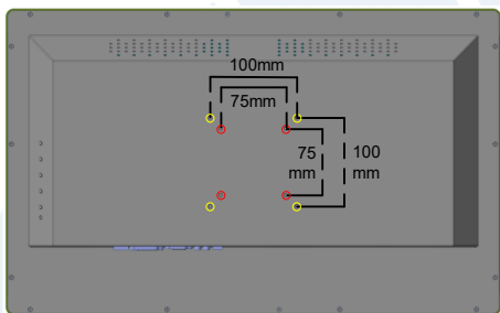
Illustration of Touch Monitor VESA Mounting Interface
