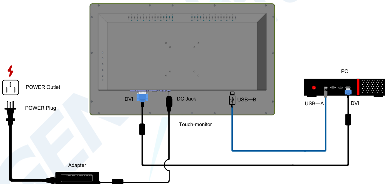
Fig 10 Touch Monitor Connection Diagram
