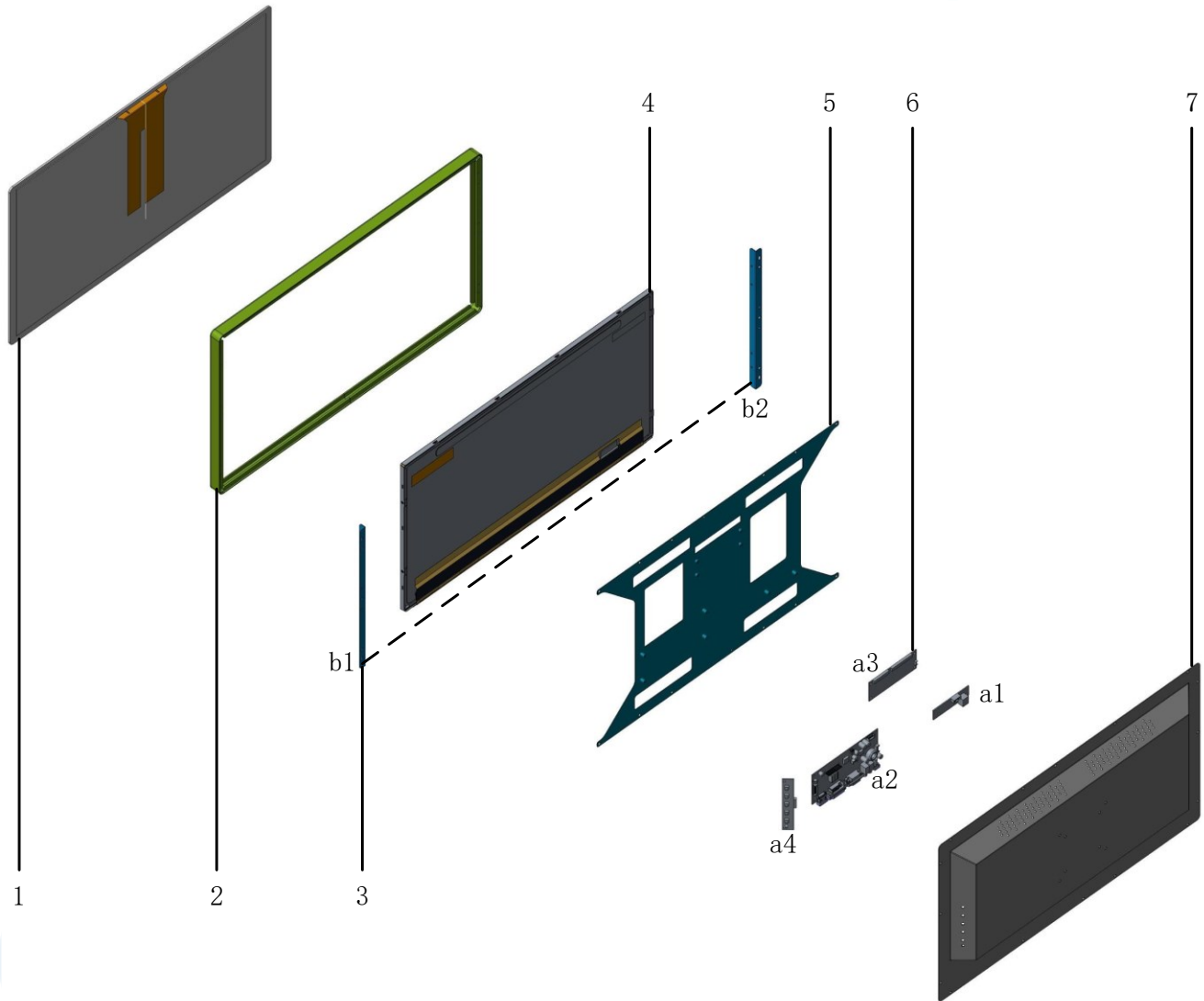
Fig 1 Cross-sectional view of the main structural components of a 23.8" closed frame touch monitor (taken as an example)
