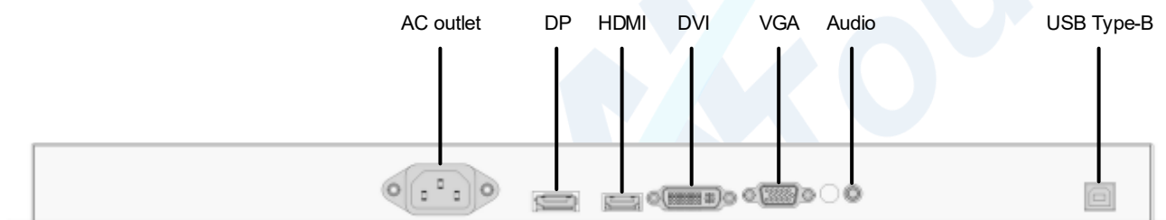
Fig 5 Bottom View of OSL323 Touchmonitor
