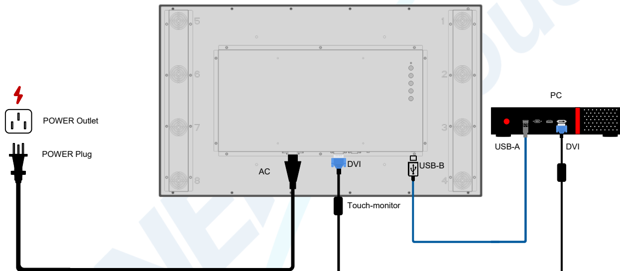
Fig 13 OSL323 Touch Monitor Connection Diagram
