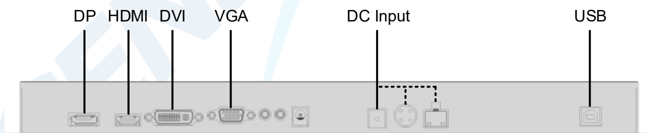
Fig 6 Bottom View of RSL276 and OSL223 Touchmonitor
