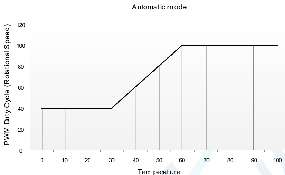
Fig 11 The relationship between temperature and fan speed
