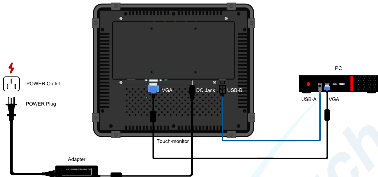
Fig 14 10.1" Touch Monitor Connection Diagram
