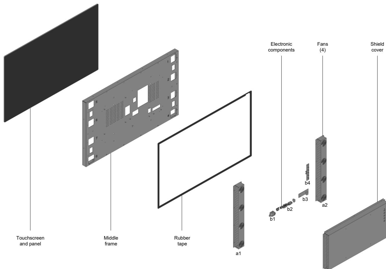
Fig 2 Cross-sectional view of the main structural components of an open frame outdoor high bright monitor
