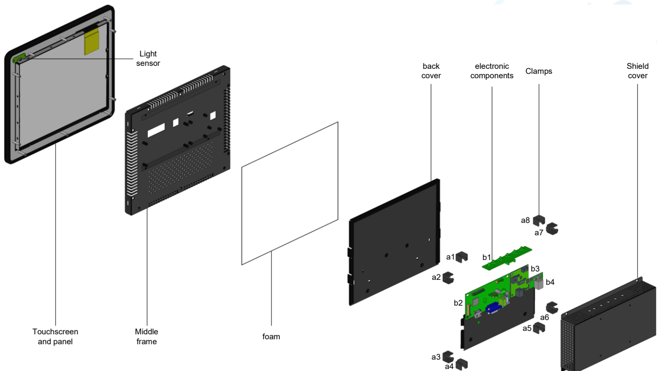
Fig 1 Cross-sectional view of the main structural components of a panel mount outdoor high bright monitor
