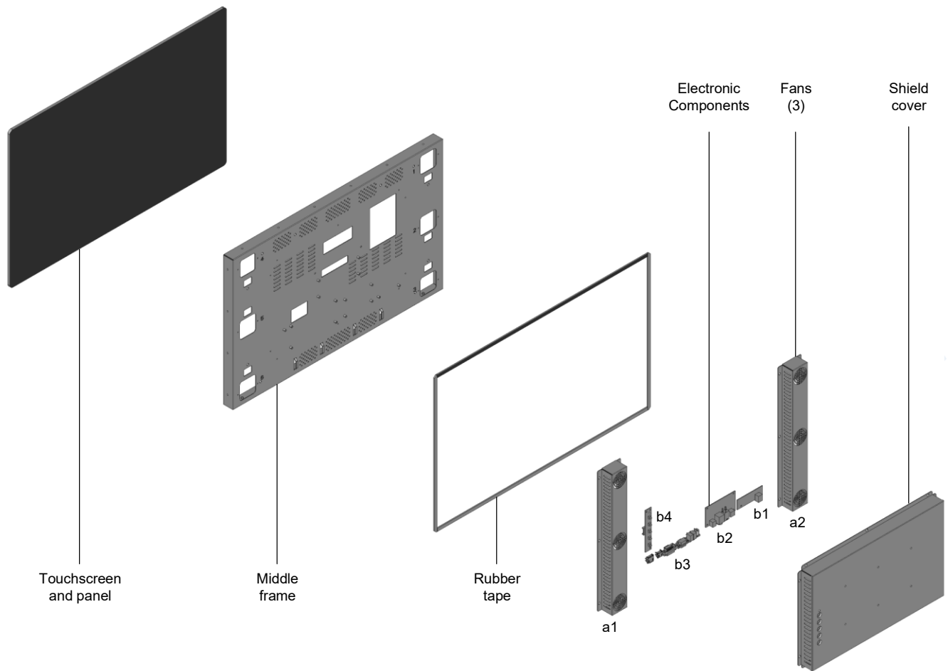
Fig 3 Cross-sectional view of the main structural components of an open frame outdoor high bright monitor
