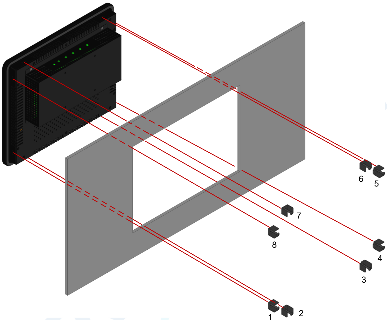
Fig 8 10.1" Embedded Mounting Installation Diagram
