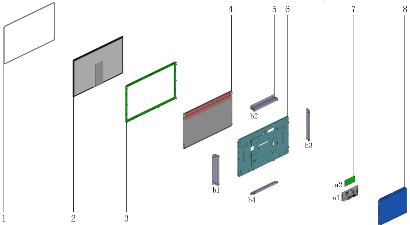
Fig 1 Cross-sectional view of the main structural components of a 21.5" rear mount touch monitor (taken as an example)
