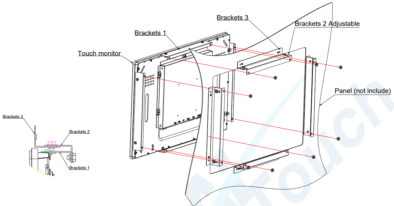
Fig 10 Cabinet Installation Diagram (Using 21.5" as an Example)
