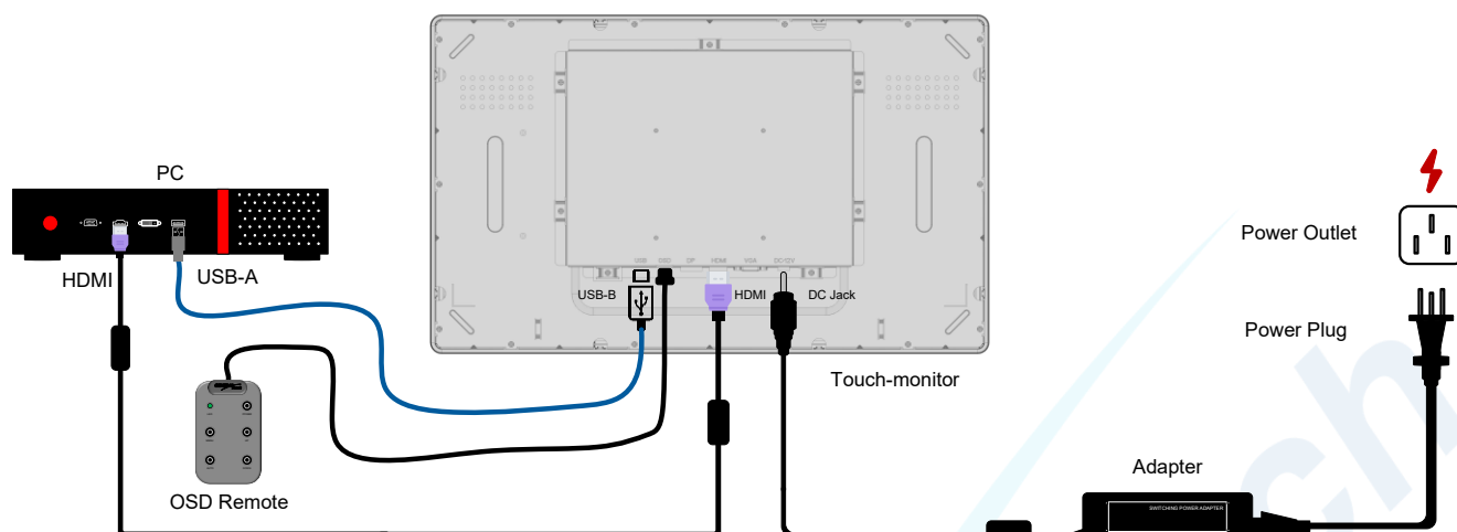
Fig 11 Touch Monitor Connection Diagram
