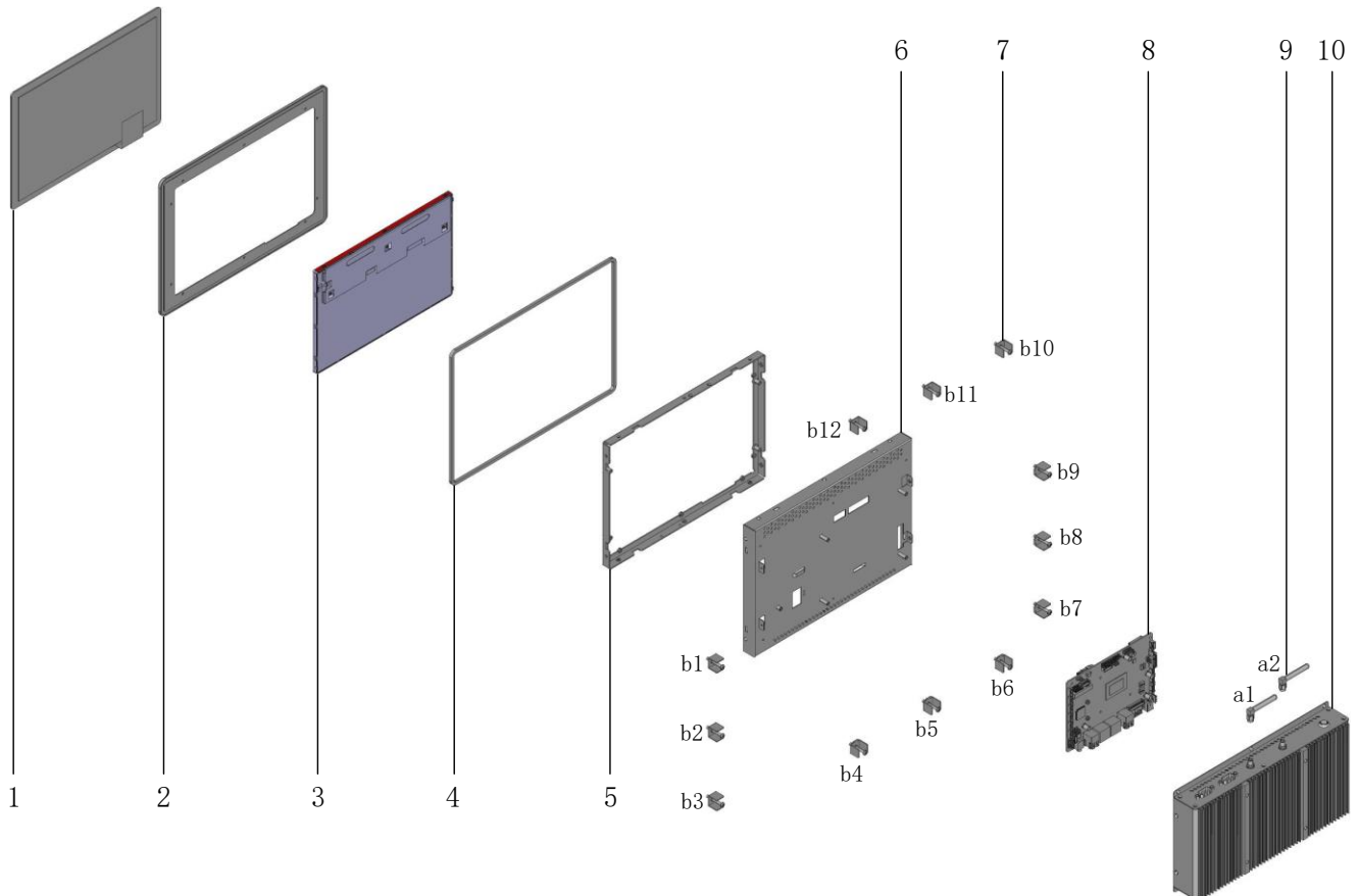
Fig 1 Cross-sectional view of the main structural components of a panel mount touch monitor
