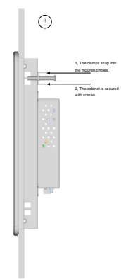
③ The clamps snap into the mounting holes on the side of the touch-monitor. Tighten the screws until they are against the cabinet.
