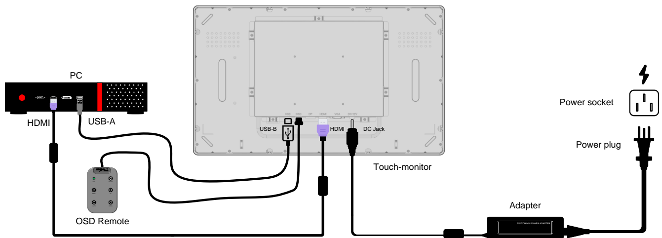
Fig 11 Touch Monitor Connection Diagram
